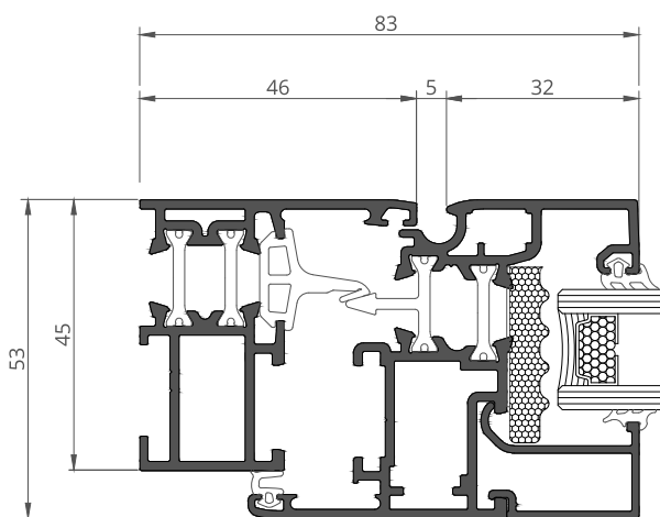
Nodo laterale/Lateral joint
