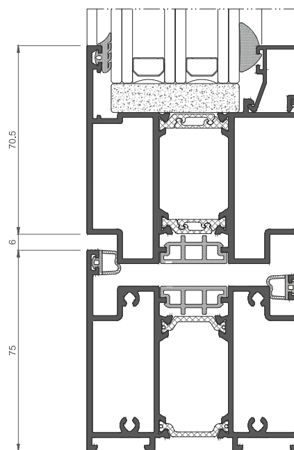
Nodo laterale con vetrocamera/Lateral joint with glazing
