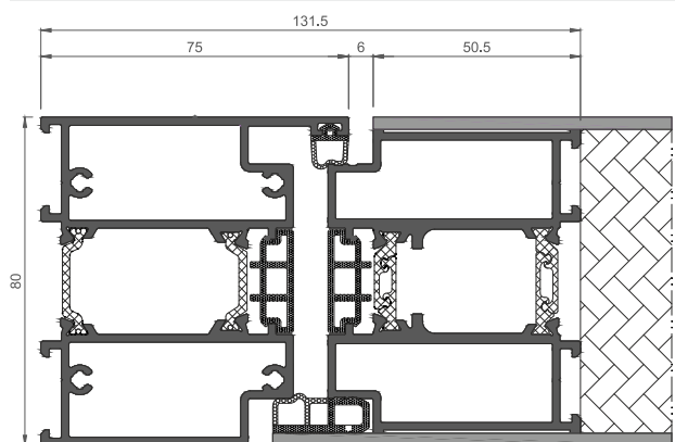
Nodo laterale con pannello Lateral joint with panel
